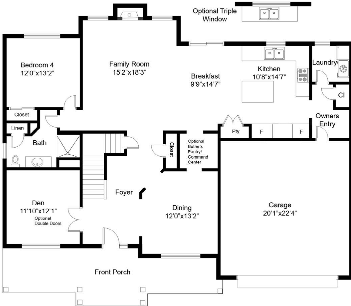
FIRST FLOOR
