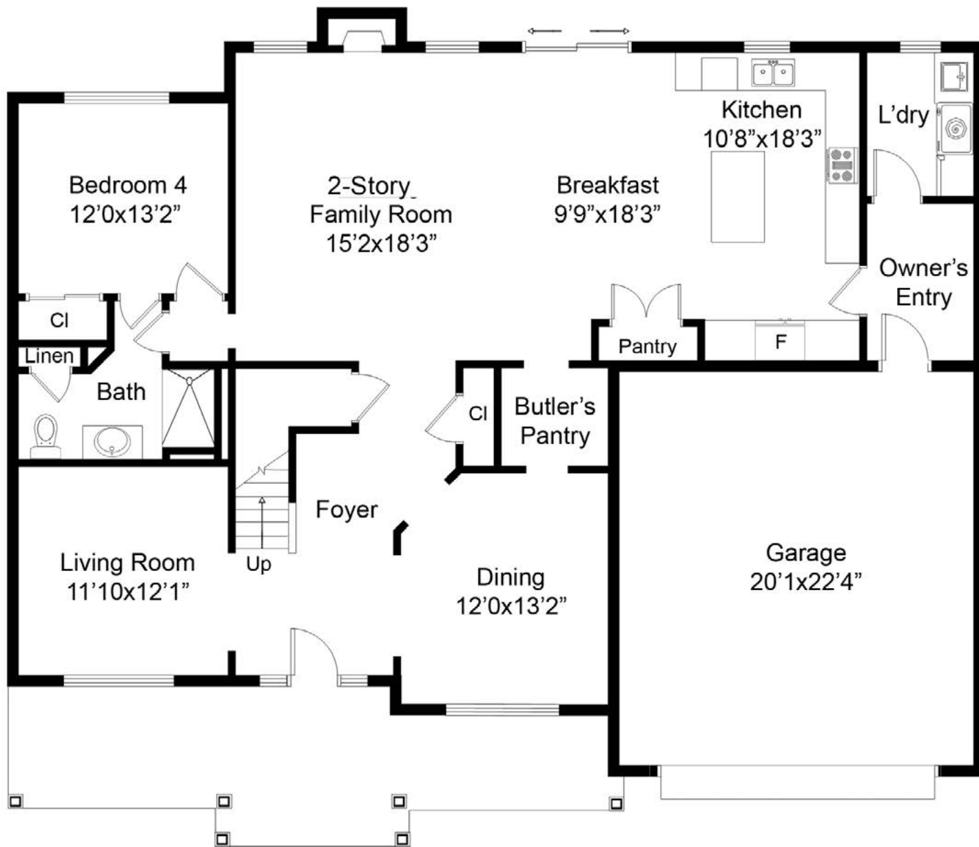
FIRST FLOOR
