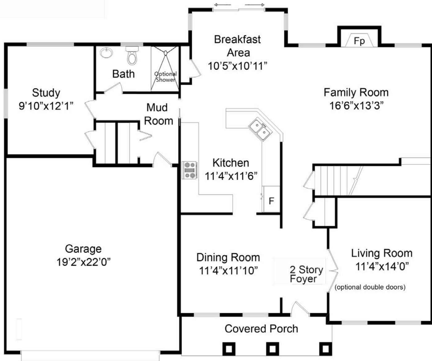
FIRST FLOOR
