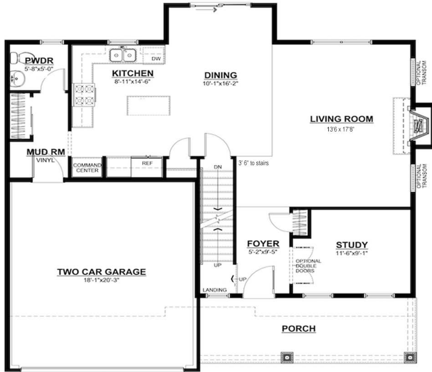
FIRST FLOOR
