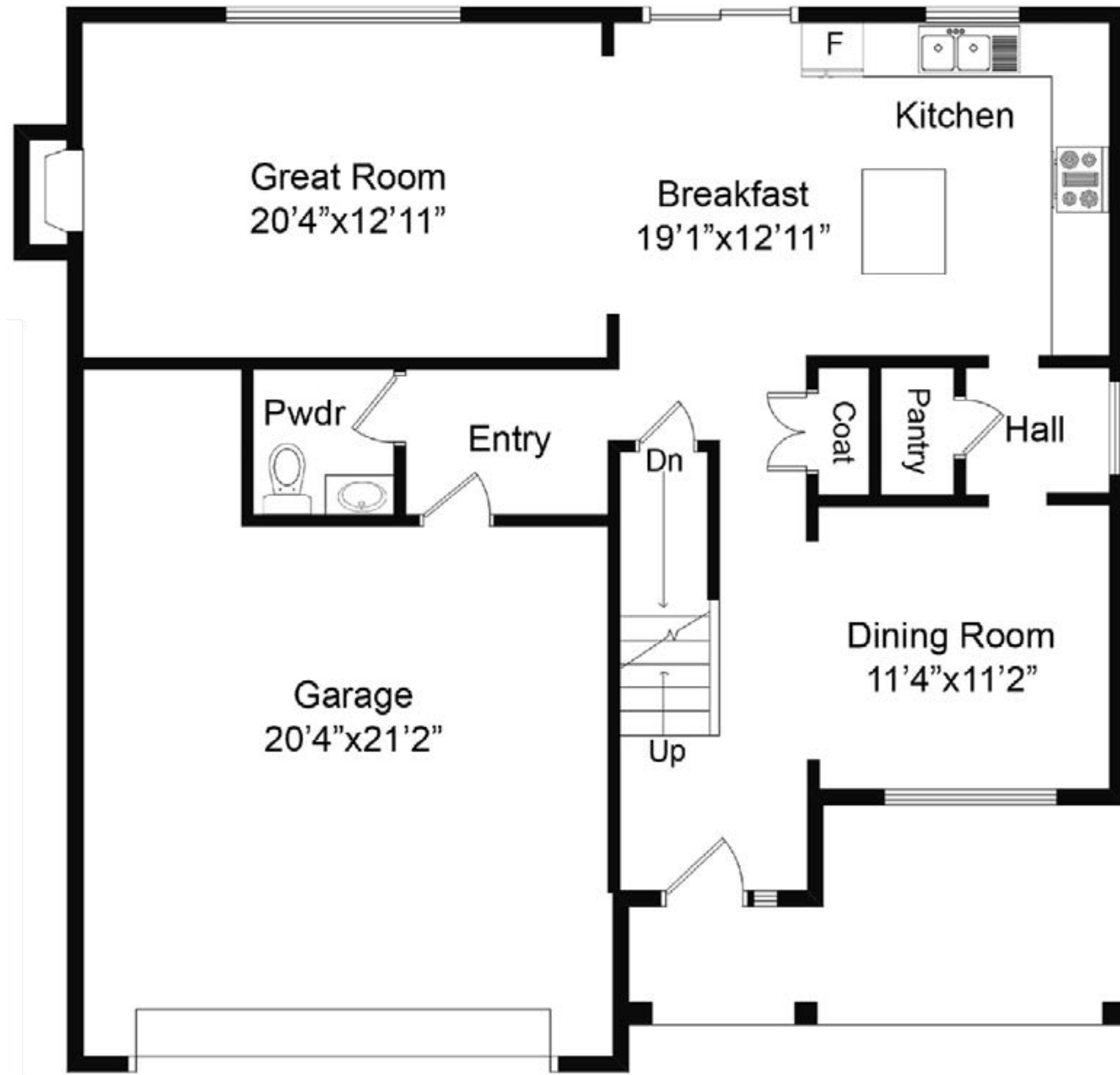
FIRST FLOOR
