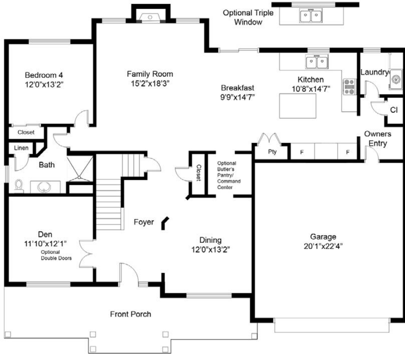
FIRST FLOOR
